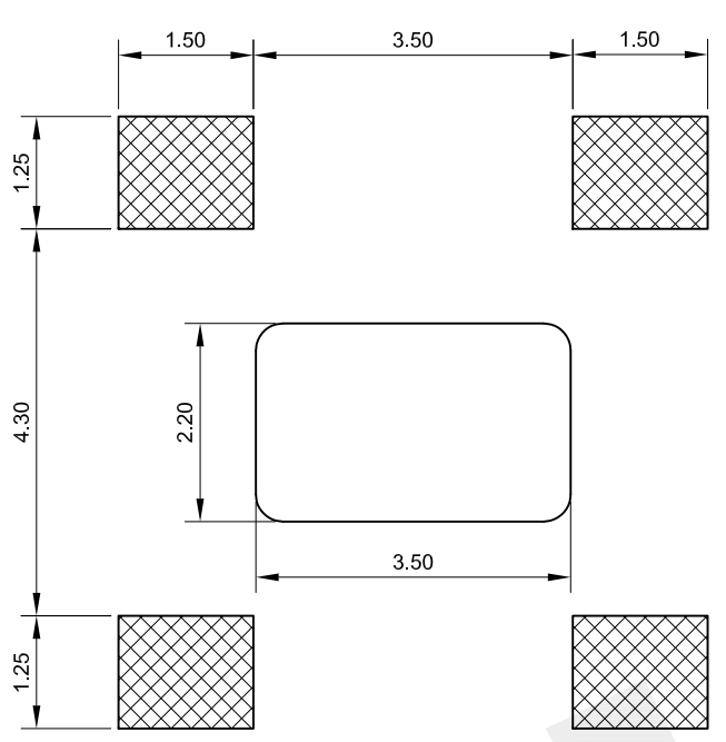
PCB LAYOUT
