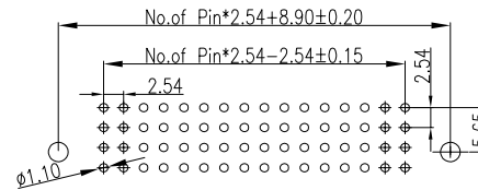
RECOMMENDED PCB LAYOUT(TOP SIDE) PCB BOARD TOLFRANCF±0.05
