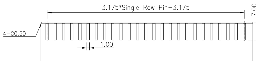
RECOMMENDED PCB LAYOUT(TOP SIDE)
