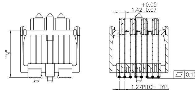
MATING HEIGHT
